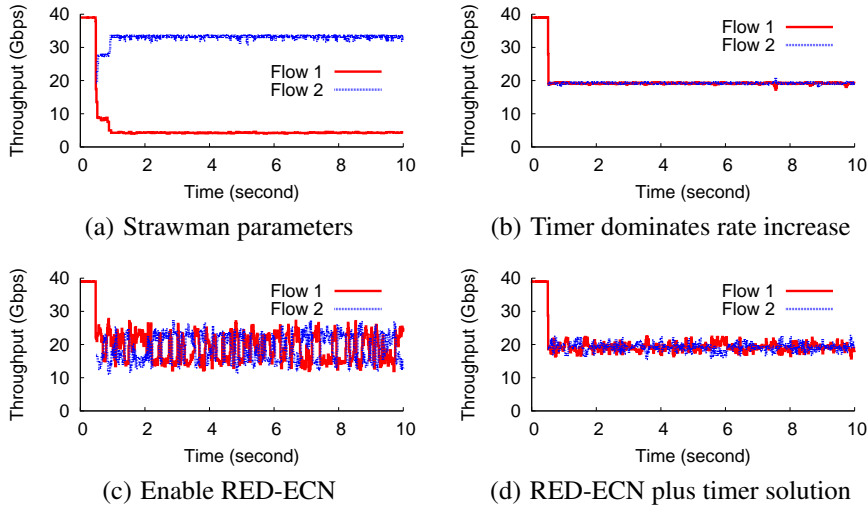
Figure 13: Validating parameter values with testbed microbenchmarks
